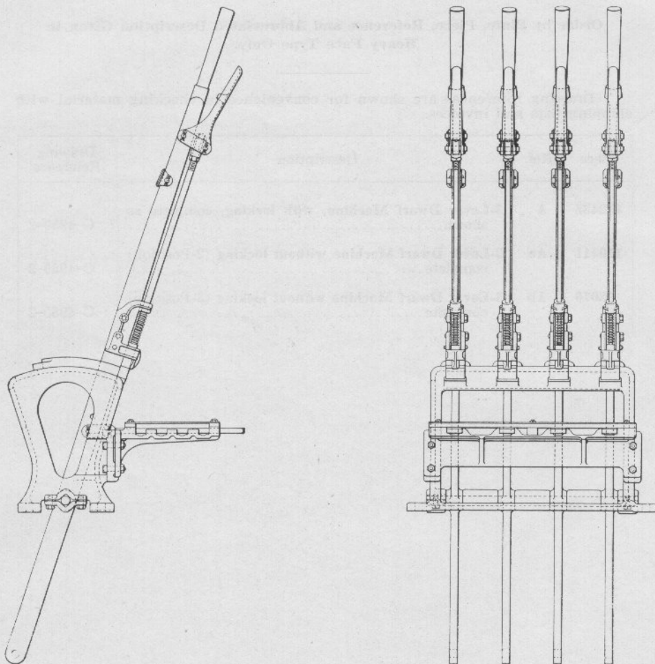
THE DWARF INTERLOCKING MACHINE ARRANGED FOR CONNECTIONS BELOW FLOOR
